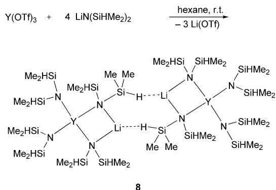
Scheme 2. Synthesis of {Y[N(SiHMe 2 ) 2 ] 4 Li} 2 8 from yttrium(III) triflate in hexane.
