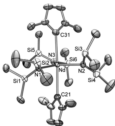
Figure 1. Molecular structure of \text{Nd}[\text{N}(\text{SiHMe}_2)_3](\text{nhc})_2 ( 4b ) shown with atomic displacement parameters at the 50% level.
