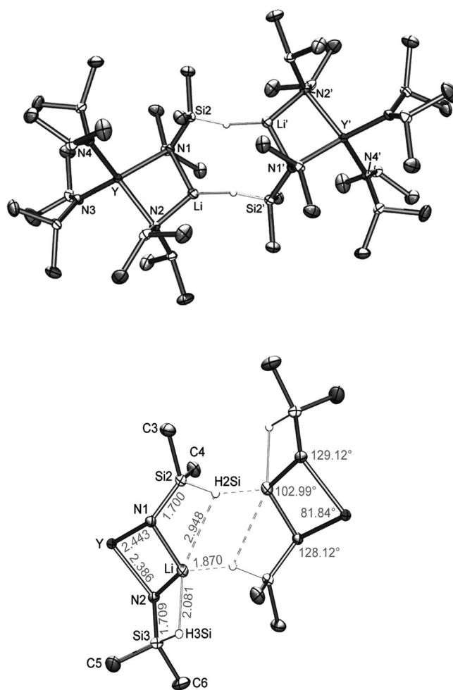
Figure 3. Molecular structure of {Y[N(SiHMe 2 ) 2 ] 4 Li} 2 ( 8 ) shown with atomic displacement parameters at the 50% level (top); Li⋯Si–H secondary interactions in 8 causing dimerization; interatomic distances are given in Å (bottom). Symmetry operation for 2 nd molecule is 1 – x, 2 – y, 1 – z.
