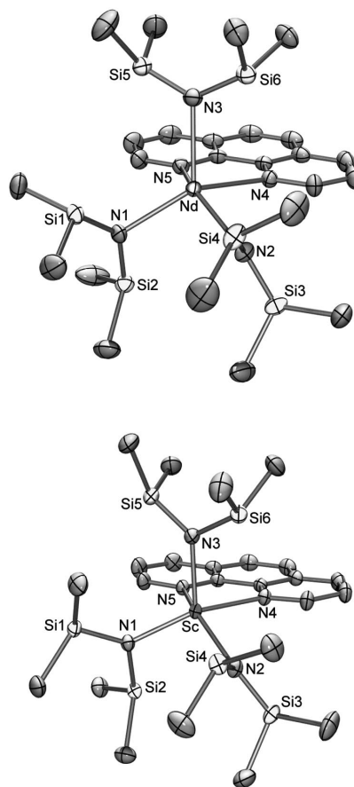
Figure 2. Molecular structures of \text{Sc}[\text{N}(\text{SiHMe}_2)_3](\text{phen}) ( 7d , bottom) and \text{Nd}[\text{N}(\text{SiHMe}_2)_3](\text{phen}) ( 7b , top) shown with atomic displacement parameters at the 50% level.
