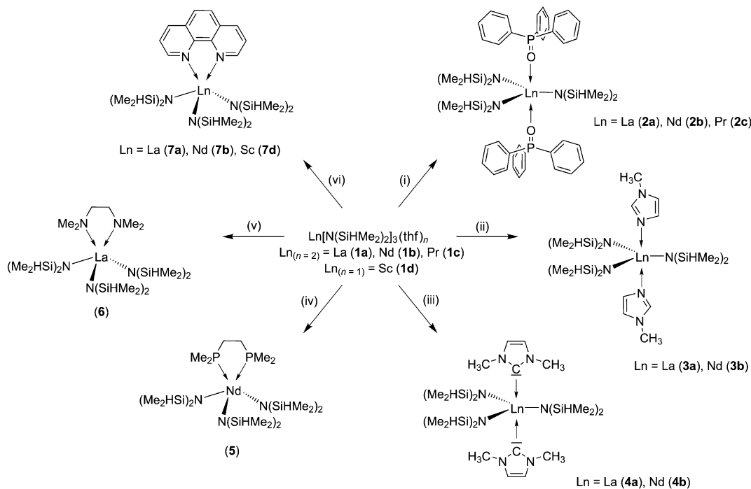
Scheme 1. Reaction of \text{Ln}[\text{N}(\text{SiHMe}_2)_2]_3(\text{thf})_n with donor molecules; (i) 2 equiv. \text{O}=\text{PPh}_3 , toluene/hexane, 12 h at ambient temp. and 1 h at 60^\circ\text{C} ; (ii) 2 equiv. N -methylimidazole, toluene/hexane, 12 h at ambient temp. and 1 h at 60^\circ\text{C} ; (iii) 2 equiv. 1,3-dimethylimidazolin-2-ylidene, thf, ambient temp.; (iv) 1,2-bis(dimethylphosphanyl)ethane, hexane, 20 min at 60^\circ\text{C} and 12 h at ambient temp.; (v) tmeda, hexane, 72 h ambient temp.; (vi) 1,10-phenanthroline, toluene, 12 h at 40^\circ\text{C} .
